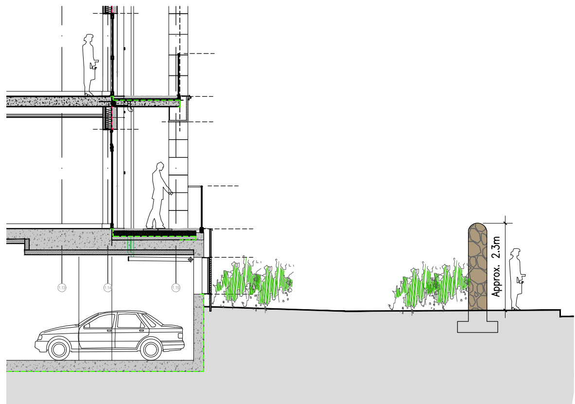
4 Proposed Boundary Treatment from Murphystown Way Section 1:100
