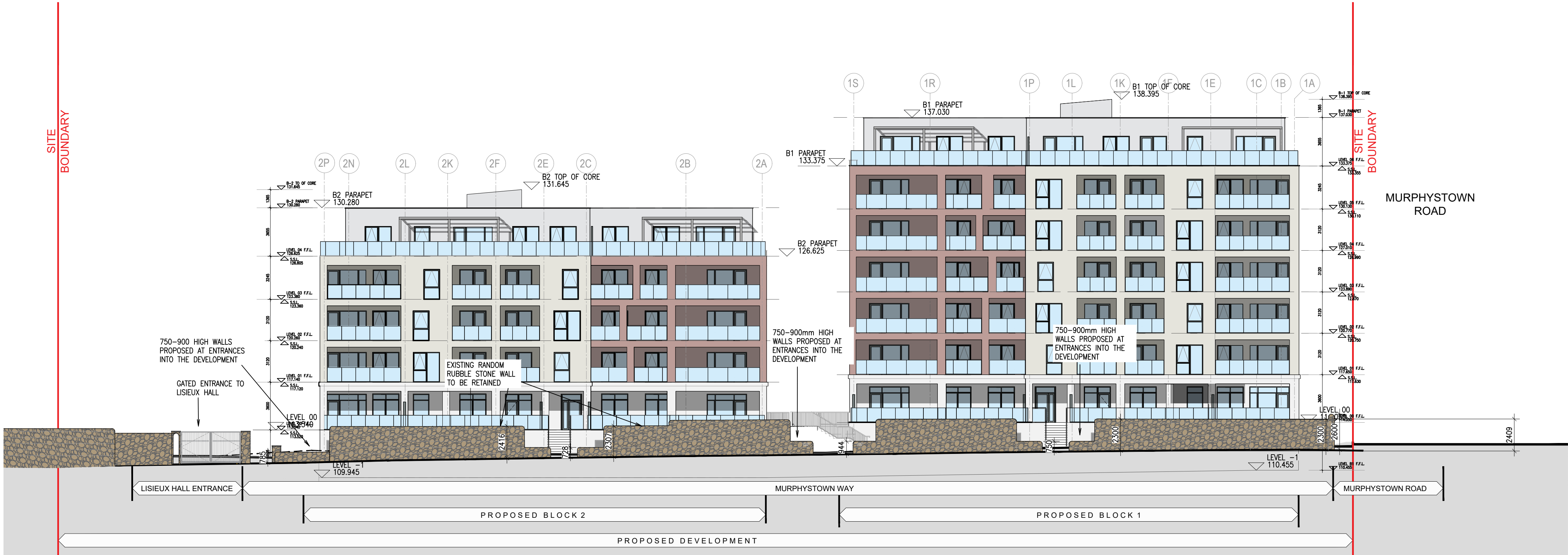
3 Proposed Boundary Treatment from Murphystown Way 1:200
